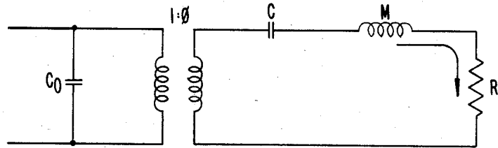
FIG. 2. PRIOR ART
